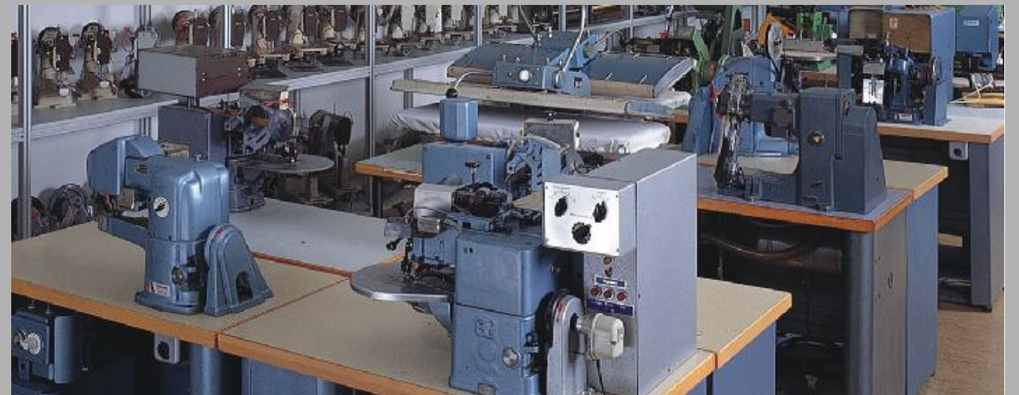
Adler 105-MO 25 single-needle heavy-duty barrel-shuttle arm-type sewing machine with special guide for making Moccasin-beads.
